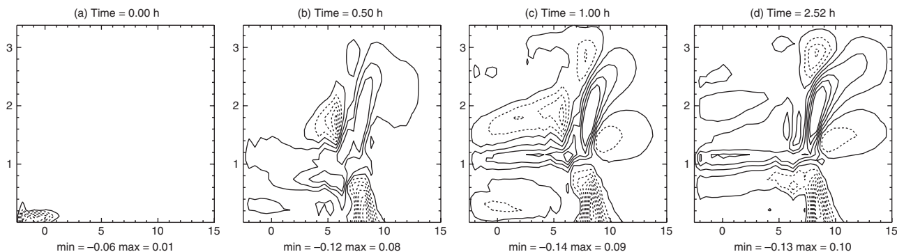
Figure 5. Contours showing the evolution of potential temperature for the optimal perturbation of experiment 1 at selected times. Solid contours are positive and dashed contours are negative. The contour interval is 0.0075 in (a) and 0.015 in (b)–(d).
