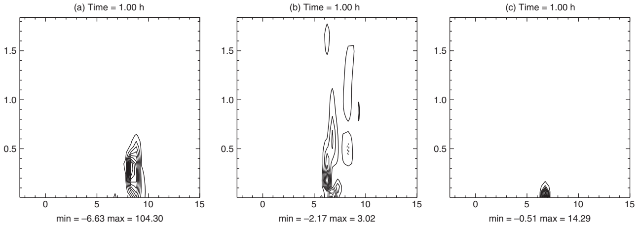
Figure 11. Contours of the dominant tendency terms in the energy equation (Eq. (9)). (a) -\langle \alpha \theta' u' \frac{\partial \bar{\theta}}{\partial x} \rangle^* . (b) -\langle u' w' \frac{\partial \bar{u}}{\partial z} \rangle^* . (c) -\langle u' u' \frac{\partial \bar{u}}{\partial x} \rangle^* .
