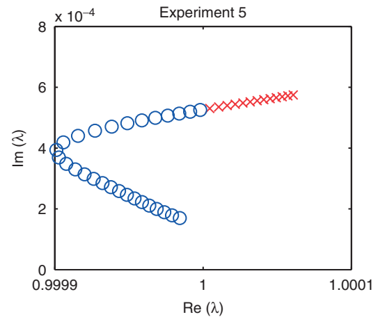
Figure 8. Example of determining the importance of specific terms in the momentum equation to the growth mechanism. In this example the term \partial p'/\partial x is multiplied by a factor \gamma , which is varied between 1 and 0 in steps of 0.025. Circles (o) indicate a stable model regime and crosses (x) mark an unstable one. This figure is available in colour online at wileyonlinelibrary.com/journal/qj
