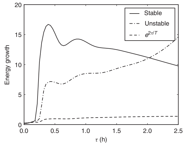
Figure 3. Kinetic energy growth factor; curves are as in Figure 2. The dashed line denotes the initial kinetic energy of the optimal initial conditions (for which E_k(t=0, \tau) is equal to one) times an exponential growth factor E_k(t=0, \tau) \exp(2\tau/T) .
