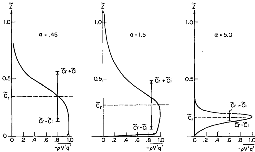
FIG. 10. The distribution (units arbitrary) of potential vorticity flux with \bar{z} for unstable eigenmodes of the usual Charney problem (with r = 1 ) at various \alpha 's.
