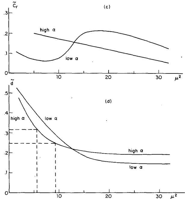
FIG. 9c. \bar{c}_r vs \mu^2 , where \bar{c}_r is the phase speed corresponding to (\alpha \bar{c}_i)_{\max} .
