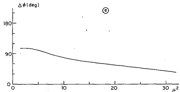
FIG. 9e. \Delta\phi vs \mu^2 , where \Delta\phi (in degrees) is the extent to which the overreflected wave associated with (\alpha \bar{c}_i)_{\max} does not satisfy Eq. (40).
