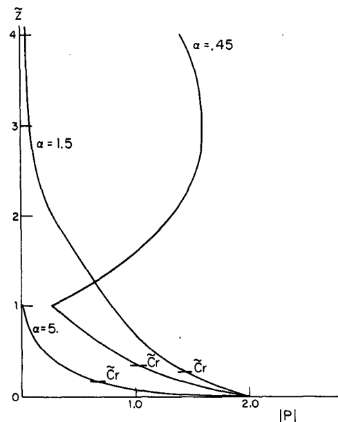
FIG. 11. The absolute value of the unstable eigenmodes as function of \bar{z} for the usual Charney problem (with r = 1 ) at those \alpha 's considered in Fig. 10.
