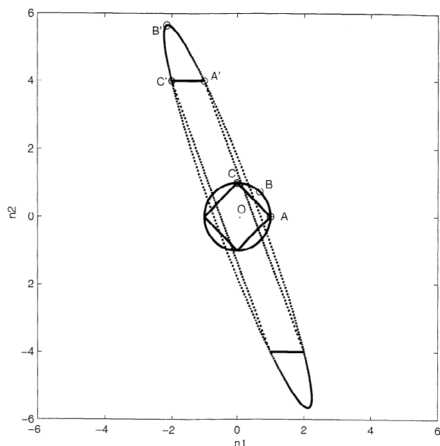
Figure 12. The result of applying the model 2 \times 2 propagator (equation A3)) to unit vectors in L_2 (the circle) and to unit vectors in L_1 (inscribed square). The optimal vector in L_2 is \mathbf{OB} , which is mapped to the evolved optimal coincident with the semimajor axis \mathbf{OB}' of length 6.05, leading to \|\Phi\|_2 = 6.05 . The optimal vector in L_1 is \mathbf{OC} , and the L_1 norm of the evolved optimal, \mathbf{OC}' , is \|\Phi\|_1 = 6 . The optimal vector in integral measure is \mathbf{OA} , and it is mapped to the evolved optimal \mathbf{OA}' with integral measure [\Phi] = 3 .
