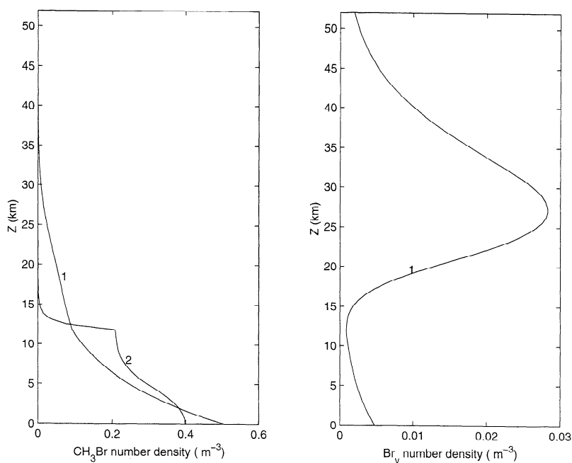
Figure 3. (left) \text{CH}_3\text{Br} number density. (right) \text{Br}_y number density. Curve 1 shows the vertical structure of the least damped \text{CH}_3\text{Br} mode with advection. The decay time of the mode is 1.48 years. Curve 2 shows the bi-orthogonal of this mode which comprises only a \text{CH}_3\text{Br} perturbation. Optimal excitation of the mode in the integral measure is achieved by placing unit \text{CH}_3\text{Br} perturbation at the ground where the bi-orthogonal has its maximum. The modes have been normalized to unity in L_2 .
