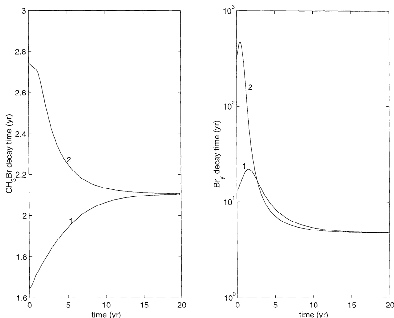
Figure 9. Relaxation timescales from an equilibrium state produced by a constant CH 3 Br source at the ground for the case of no advection. The influence of variable choice is revealed by the contrast between two cases. Curve 1 shows the instantaneous decay time of number density as a function of time from removal of the source. (left) CH 3 Br. (right) Br y . Curve 2 shows the instantaneous decay time of mixing ratio as a function of time from removal of the source.
