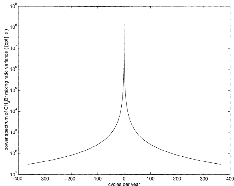
Figure 11. Power spectrum of \text{CH}_3\text{Br} mixing ratio variance averaged over the troposphere (0 – 10 km) resulting from white noise forcing of \text{CH}_3\text{Br} at the ground. The frequencies shown correspond to periods longer than a day. The peak response occurs for stationary forcing, and the response falls off rapidly with increasing frequency. Vertical advection is included.
