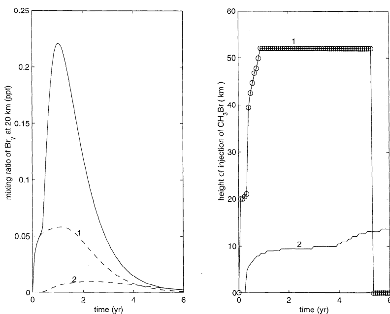
Figure 4. (left) Optimal growth of \text{Br}_y mixing ratio (parts per trillion (ppt)) at 20 km as a function of optimization time. Optimization time is defined as the time selected to calculate the maximum possible growth (the optimal growth) in the system as quantified by the selected measure of chemical perturbations, which is here the mixing ratio of \text{Br}_y at 20 km. Only \text{CH}_3\text{Br} initial perturbations are considered. The amount released at the ground over a grid interval \Delta z is equivalent to 1 ppt over the first 2 km ( 4.8 \times 10^{16} \text{ m}^{-2} ). Both advection and diffusion are included. Dashed curve 1 shows the time evolution of the 2 month optimal perturbation. Dashed curve 2 shows the time evolution of the 6 year optimal perturbation, which is initially at the ground. (right) Height (kilometers) of the optimal \text{CH}_3\text{Br} perturbation is shown as a function of optimization time (curve 1). Height (kilometers) of the initial perturbation in \text{CH}_3\text{Br} that leads to the least response in \text{Br}_y mixing ratio at 20 km is shown as a function of optimization time (curve 2).
