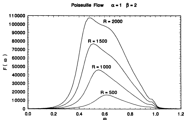
FIG. 3. The frequency response function F(\omega) in the energy norm for plane Poiseuille flow with streamwise wave number \alpha=1 and spanwise wave number \beta=2 for various Reynolds numbers R .
