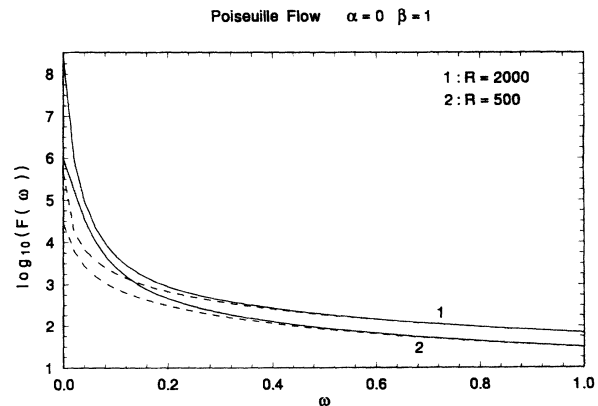
FIG. 2. The frequency response function F(\omega) in the energy norm for plane Poiseuille flow with streamwise wave number \alpha=0 and spanwise wave number \beta=1 . Curve 1 corresponds to Reynolds number R=2000 ; curve 2 to R=500 . The dashed curves show the frequency response that would result if the operator were interpreted as a normal operator.
