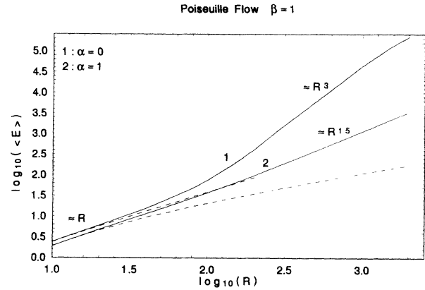
FIG. 1. Variation of ensemble average energy as a function of Reynolds number R for plane Poiseuille flow. The full line indicates the variance of the non-normal operator. The dashed line represents the variance that would result if the operator were interpreted as a normal operator. Both cases are for spanwise wave number \beta=1 . Curve 1 is for streamwise wave number \alpha=0 , and curve 2 for \alpha=1 .
