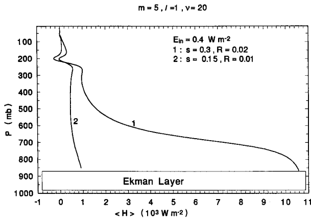
FIG. 16. Distribution of the heat flux with height for zonal wave-number 5 and meridional wavenumber l = 1 . The basic state is the same as in Fig. 1. For the winter months s = 0.3 , R = 0.02 , for the summer months s = 0.15 , R = 0.01 , and E_{in} = 0.4 \text{ W m}^{-2} .
