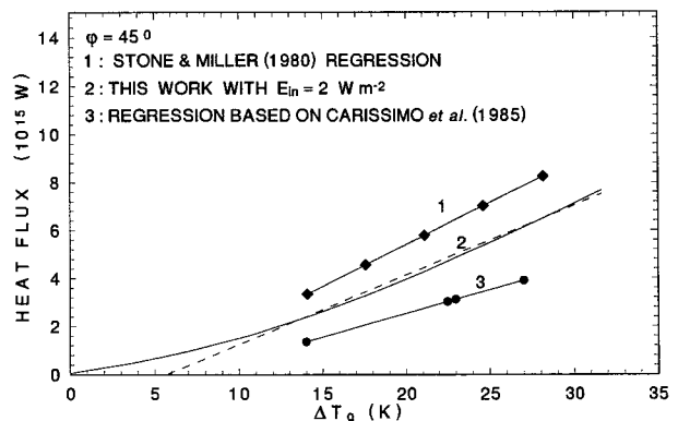
FIG. 18. Variation of the total ensemble average heat flux at 45^\circ\text{N} as a function of \Delta T_g . Curve 2 is the result of stochastic forcing of the model atmospheric jet for k = 2 , l = 2 , R = 0.01 , \nu = 20 \text{ m}^2 \text{ s}^{-1} , and E_{in} = 2 \text{ W m}^{-2} . The dash curve is a linear fit. Curve 1 has been compiled by Stone and Miller (1980) based on observations of seasonally averaged heat flux. Curve 3 is based on the seasonally averaged observations of Carissimo et al. (1985).
