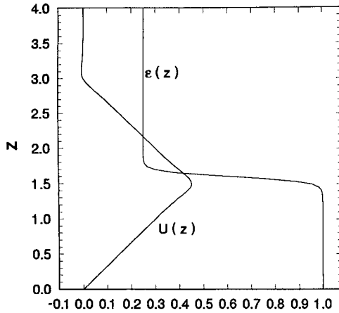
FIG. 1. The nondimensional mean flow velocity and Brunt-Väisälä frequency variation with height. The nondimensional shear s = 0.3 corresponds to a dimensional maximum zonal velocity of 35 \text{ m s}^{-1} , and \epsilon in the troposphere corresponds to Brunt-Väisälä frequency N = 10^{-2} \text{ s}^{-1} . The tropopause is located at nondimensional height z = 1.5 .
