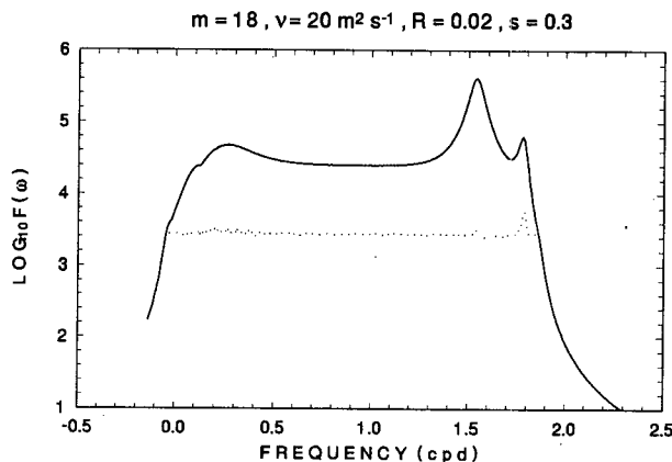
FIG. 9. The power spectrum as a function of frequency (in cycles per day) for global zonal wavenumber 18. This spectrum is obtained from stochastic forcing of a baroclinic jet with nondimensional shear parameter s = 0.3 , linear damping of R = 0.02 (corresponding to an e -folding time of 6 days), and vertical diffusion coefficient \nu = 20 \text{ m}^2 \text{ s}^{-1} . The nondimensional meridional wavenumber is l = 1 . The dotted line corresponds to the maintained variance obtained from the equivalent normal evolution operator. The higher-frequency peak corresponds to the upper-level variance concentrated near the tropopause.
