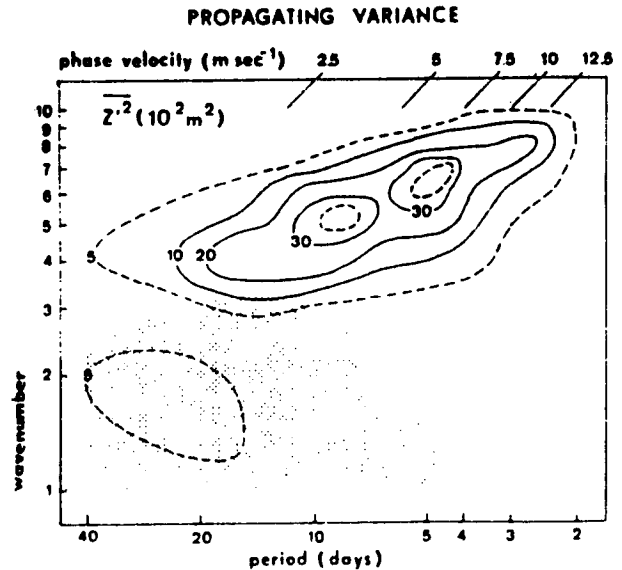
FIG. 5. Power spectrum of geopotential at 500 mb and 50^\circ\text{N} averaged over the winter seasons between 1972 and 1973 (from Fraedrich and Böttger 1978).
