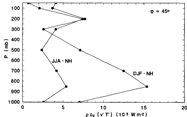
FIG. 7. The distribution of the zonally and seasonally averaged transient heat flux for latitude 45^\circ\text{N} , from the values given by Oort and Peixoto (1983). DJF denotes the winter months; JJA denotes the summer months.
