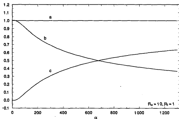
FIG. 7. Contributions to the energy balance in a constant shear flow. (a) Average perturbation energy input \epsilon ; (b) ensemble-average perturbation energy dissipation D ; (c) average energy lost, through Reynolds stress, to the mean flow F , as a function of shear. The bandpass is 1 < r_0 < 10 .
