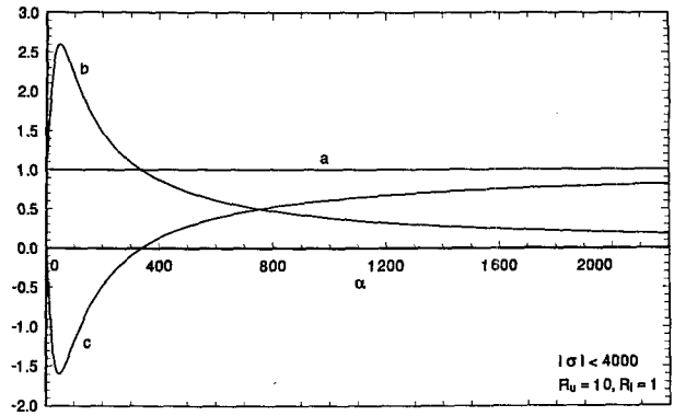
FIG. 8. Contribution to the energy balance in a deformation flow. (a) Average perturbation energy input \epsilon ; (b) ensemble-average perturbation energy dissipation D ; (c) average energy lost, through Reynolds stress, to the mean flow F , as a function of \alpha for a deformation flow with wave-front-normal directions limited by |\sigma| < 4000 . The bandpass is 1 < r_0 < 10 .
