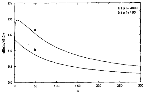
FIG. 5. The ensemble-average perturbation energy density at \alpha normalized by the ensemble-average perturbation density at zero \alpha as a function of \alpha for deformation flows. The wave-front-normal directions are limited by (a) |\sigma| < 4000 ; (b) |\sigma| < 100 . The bandpass is 1 < r_0 < 10 .
