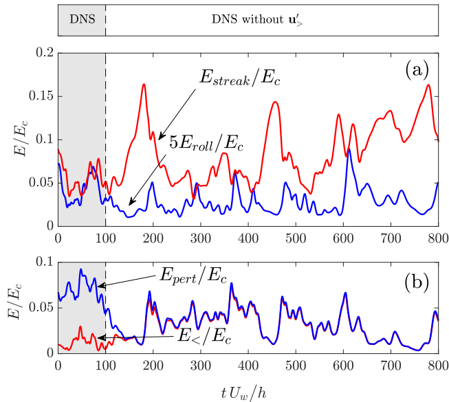
Figure 3: (a): Same as Fig. 2 but now the complement \mathbf{u}'_> is removed with the same protocol. The turbulence sustains in DNS with the full perturbation field converging to a single Lyapunov vector of the fluctuating mean flow.
