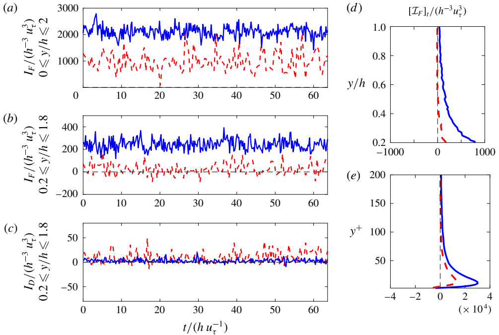
FIGURE 15. (Colour online) (a–c) Time series of the contribution to the time rate of change of streamwise square vorticity \int dy [\Omega_x^2/2]_z by perturbation torques, I_F , and by advection of streamwise mean vorticity by the mean flow, I_D , for NS940 (solid) and RNL940 (dashed). (a) I_F over the whole channel, 0 \leq y/h \leq 2 ( I_D = 0 in this case). The time mean I_F is 2103.6h^{-3}u_\tau^3 for NS940 and 982.8u_\tau^3 for RNL940. (b) I_F over the outer layer, 0.2 \leq y/h \leq 1.8 . The time mean I_F for this region is 242.5h^{-3}u_\tau^3 for NS940 and only 28.7h^{-3}u_\tau^3 for RNL940. (c) I_D for the outer layer 0.2 \leq y/h \leq 1.8 . The time mean I_D is 2.9h^{-3}u_\tau^3 for NS940 and 11.2h^{-3}u_\tau^3 for RNL940. These figures show that in NS940 and RNL940 the roll is maintained locally by the perturbation Reynolds stresses. (d,e) Cross-stream structure of the time-averaged contribution to the streamwise mean vorticity generation from perturbation Reynolds-stress-induced torques [\mathcal{I}_F]_t(y) .
